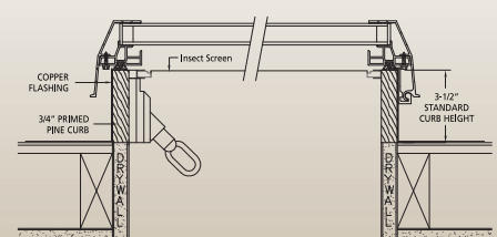
Cut Flush Curb
