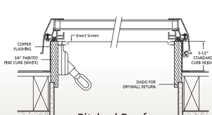
Pitched Roof Drop-In Curb
