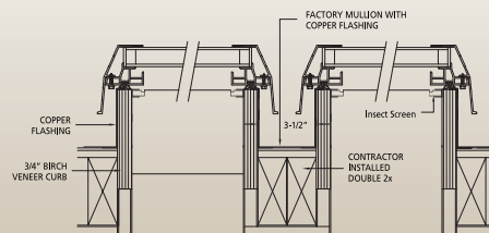
Factory Mullied Curb
