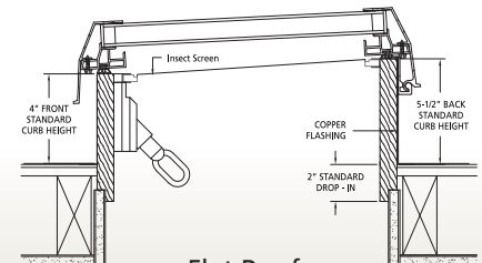
Flat Roof Drop-In Curb
