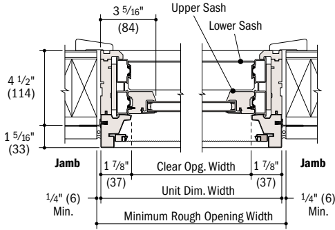
Horizontal Section
